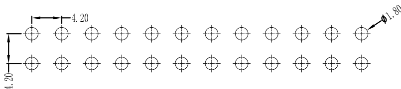
PCB LAYOUT
